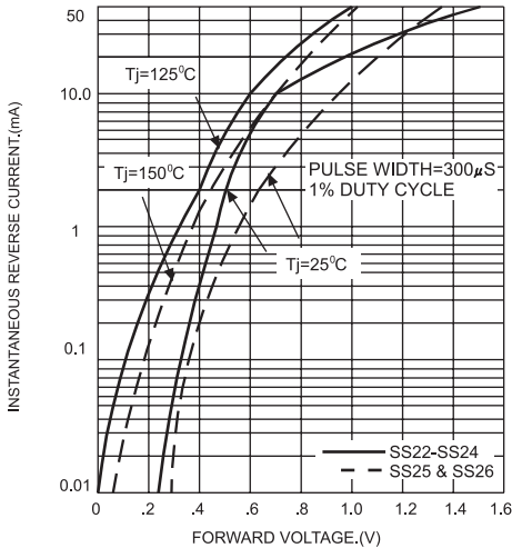
FIG.3-TYPICAL FORWARD CHARACTERISTICS
