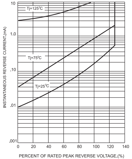
FIG.5-TYPICAL REVERSE CHARACTERISTICS
