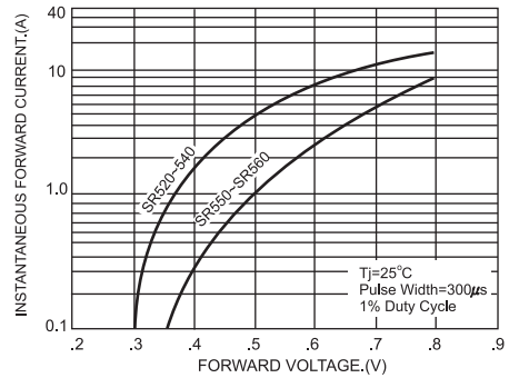
FIG.4-TYPICAL FORWARD CHARACTERISTICS
