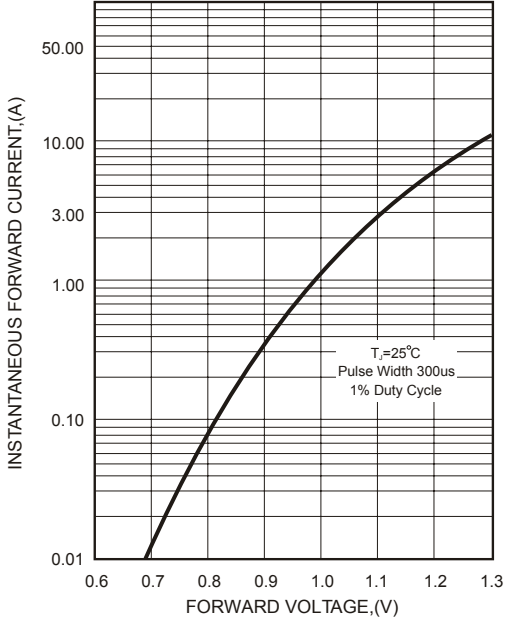
FIG.1-TYPICAL FORWARD CHARACTERISTICS
